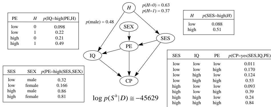
Figure 11: The a posteriori most likely network structure with a hidden variable. Probabilities shown are MAP values. Some probabilities are omitted for lack of space.
